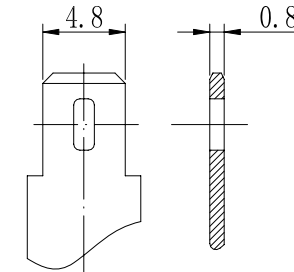
Terminal T1
